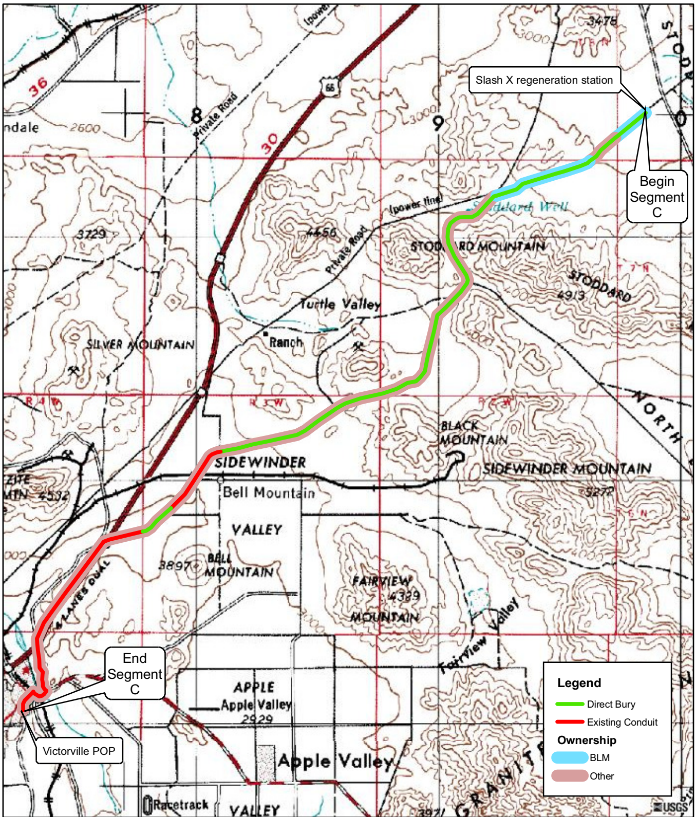
Segment C Slash X regeneration station to Victorville POP Figure 4
